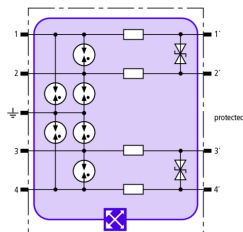
Basic circuit diagram BXT ML4 BD EX 24
